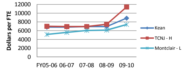
Instr. Expen. per FTE - 5-Year Trend Kean vs. NJASCU High & Low
